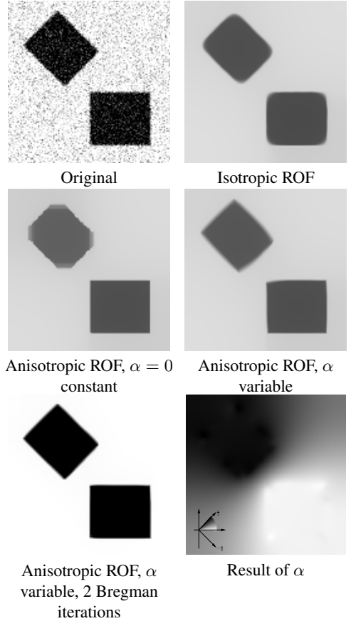
Figure 3: Reconstruction of two artificial rectangles with different methods.
